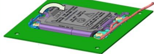
3. Close the load plate - ILM Cover should "Pop-Off"
